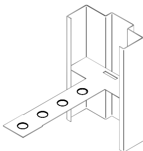
T-ANCHOR
