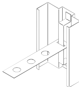
STRAP ANCHOR
