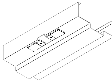
AUTO. FLUSH BOLT STRIKE W/ LIP
