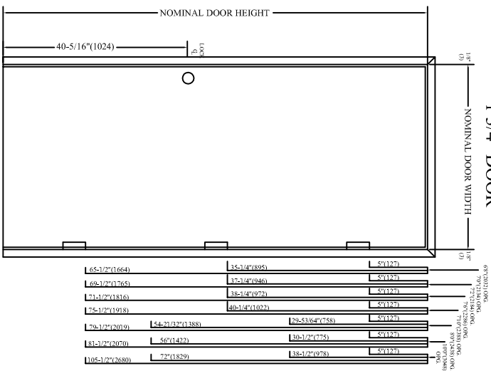
ELEVATION For 1-3/4" (44) Single Door
