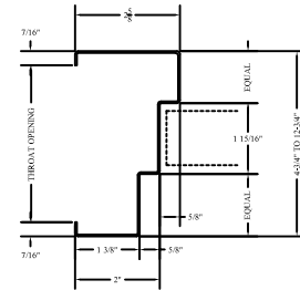
1 3/8" (35) FACE STANDARD
