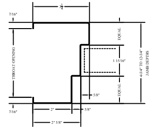
2" (51) FACE STANDARD
