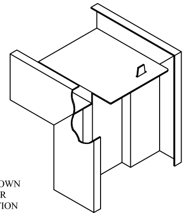
U.L. MASONRY ANCHOR (WELDED IN)
