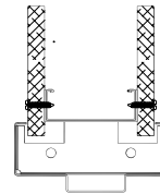
WRAP ANCHOR W/ STEEL STUDS
