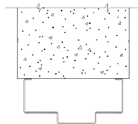
BUTT ANCHOR W/ CONC.
